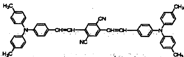
Structural formula (15)-4:
